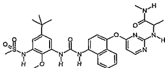
2-(4-{4-[3-(5-tert-Butyl-3-methanesulfonylamino-2-methoxy-phenyl)-ureido]-naphthalen-1-yloxy}-pyrimidin-2-ylamino)-N-methyl-propionamide;
